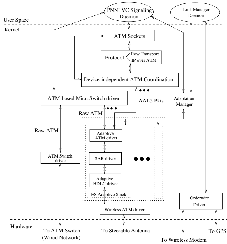
Figure 6: ES-Network Protocol Stack
