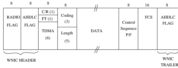
Figure 7: Basic HDLC-like Frame Format.
