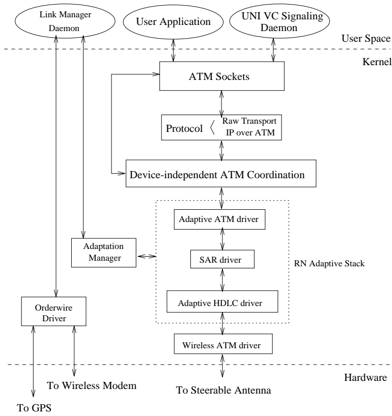
Figure 5: RN Network Protocol Stack.
