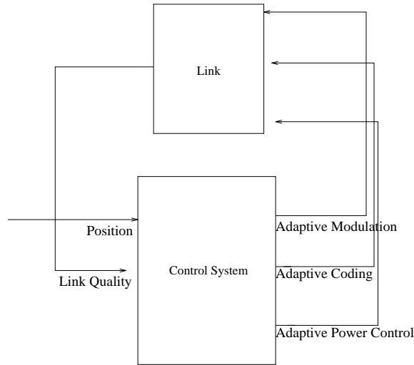
Figure 12: Adaptive Control.
