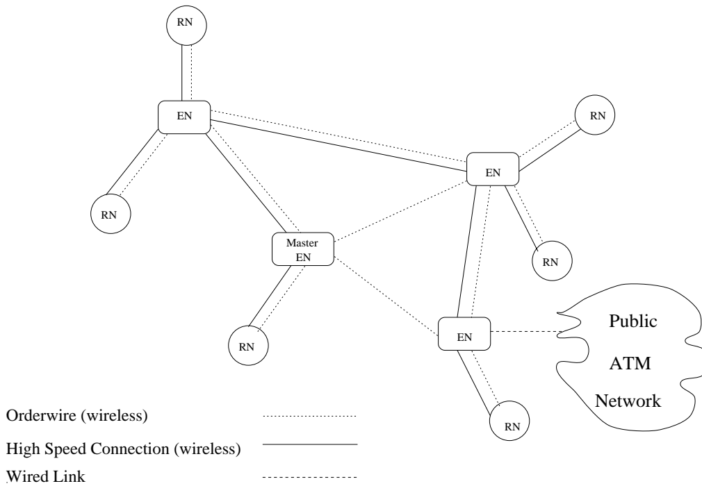
Figure 13: Example Orderwire Topology.
