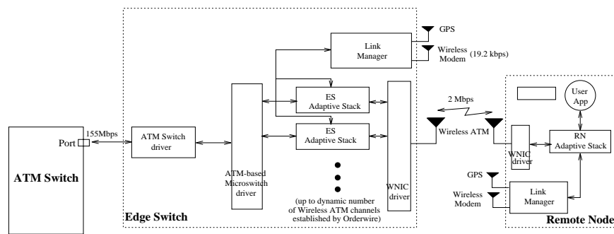
Figure 10: Detailed view of Edge Switch Connection to Remote Node.
