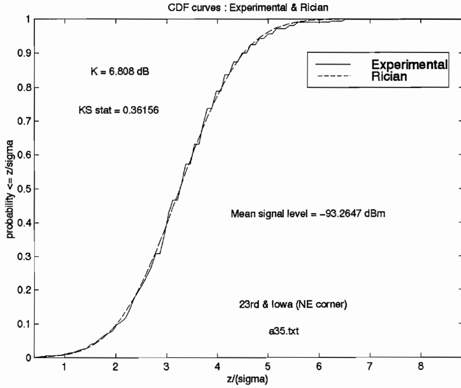
Figure 134: CDF for NE corner 23 rd and Iowa (a35) and the theoretical Rician CDF.
