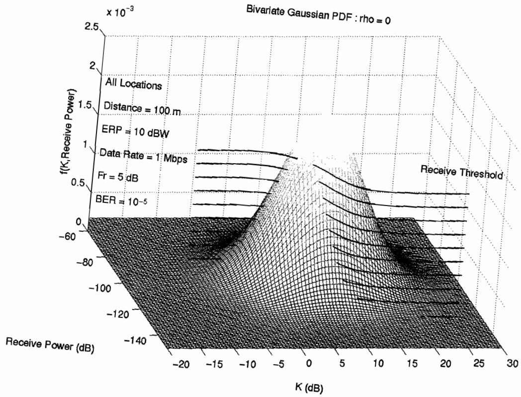
Figure 5: Bivariate Gaussian probability density function for independent K and receive power at a transmitter-receiver separation of 100m.
