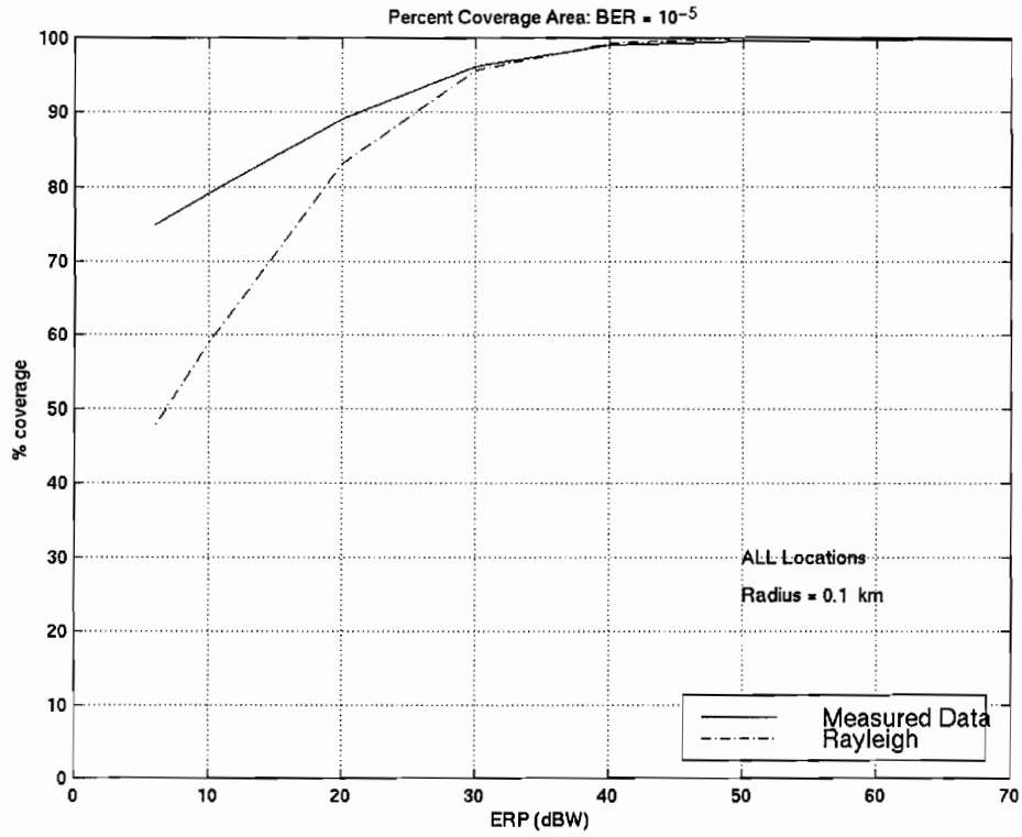
Figure 59: Percent coverage area for the actual correlated K and receive power distribution and the Rayleigh channel assumption for ALL locations with BER = 10^{-5} and a cell boundary of 100m.
