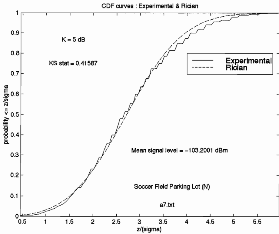
Figure 113: CDF for soccer field N parking lot (a7) and the theoretical Rician CDF.
