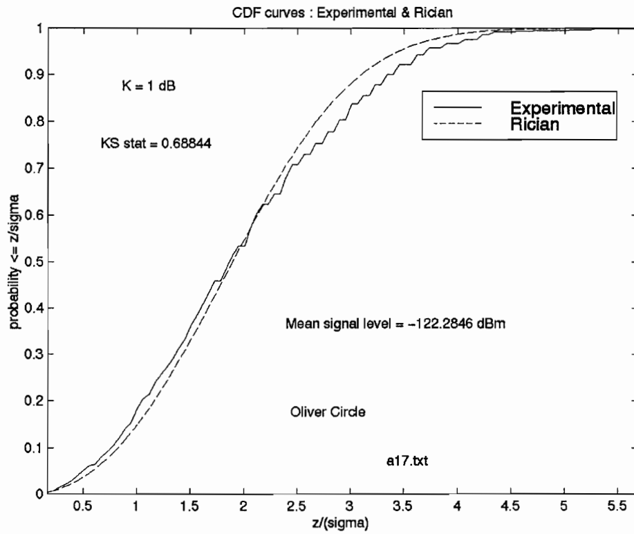
Figure 123: CDF for Oliver dormitory circle (a17) and the theoretical Rician CDF.
