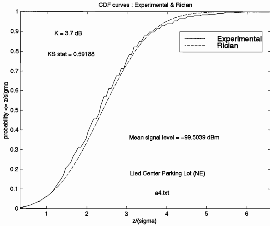
Figure 111: CDF for Lied Center NE parking lot (a4) and the theoretical Rician CDF.
