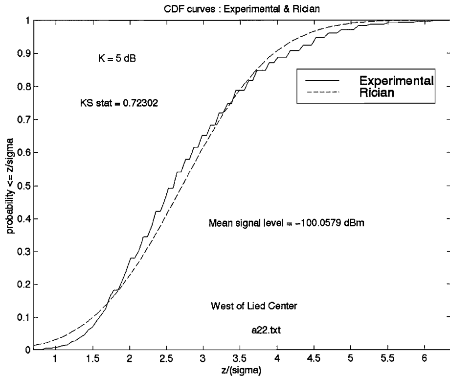
Figure 126: CDF for dirt road west of Lied Center (a22) and the theoretical Rician CDF.
