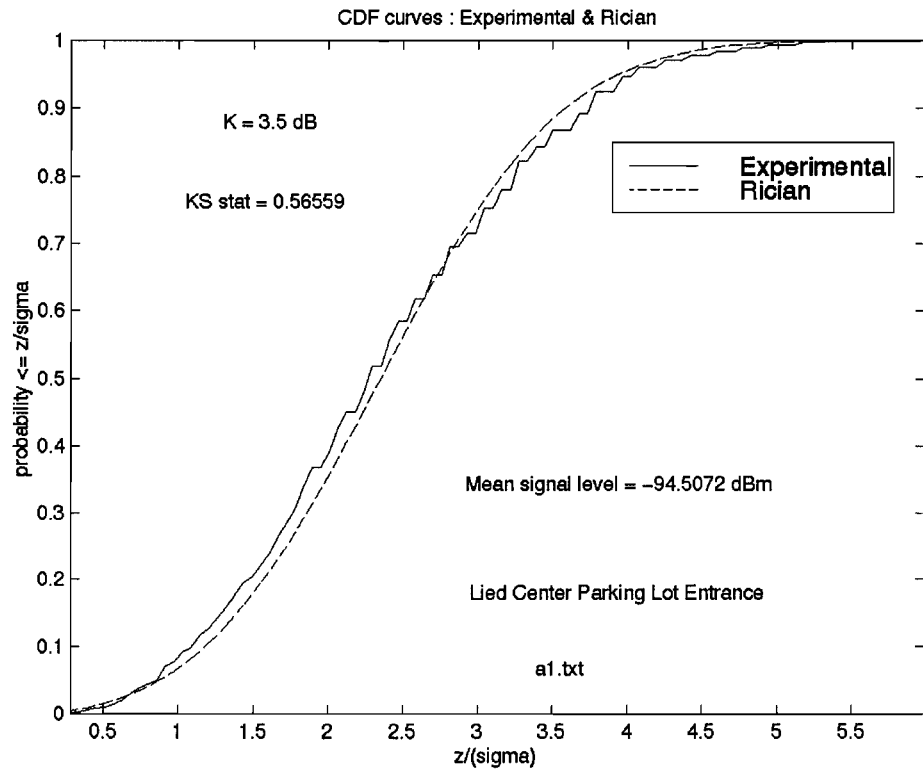
Figure 108: CDF for Lied Center parking lot entrance (a1) and the theoretical Rician CDF.
