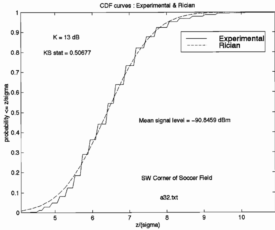
Figure 132: CDF for SW corner of soccer field (a32) and the theoretical Rician CDF.
