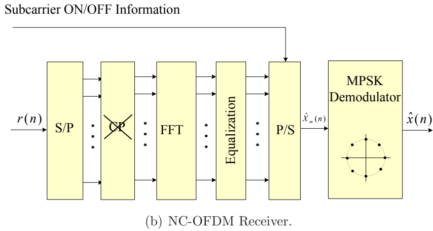
Figure 2.9. Schematic of an NC-OFDM transceiver employing null subcarrier selection block.
