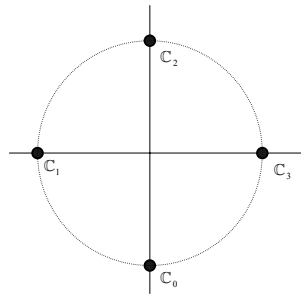
Figure 5.20. Constellation diagram for QPSK symbols.
