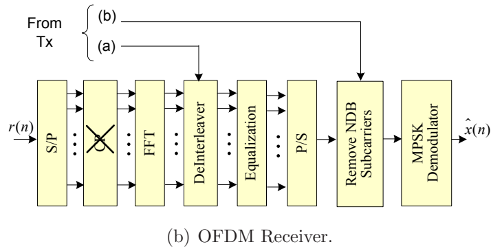
Figure 5.19. OFDM transceiver employing adaptive NDB subcarrier approach with interleaving for PAPR reduction.
