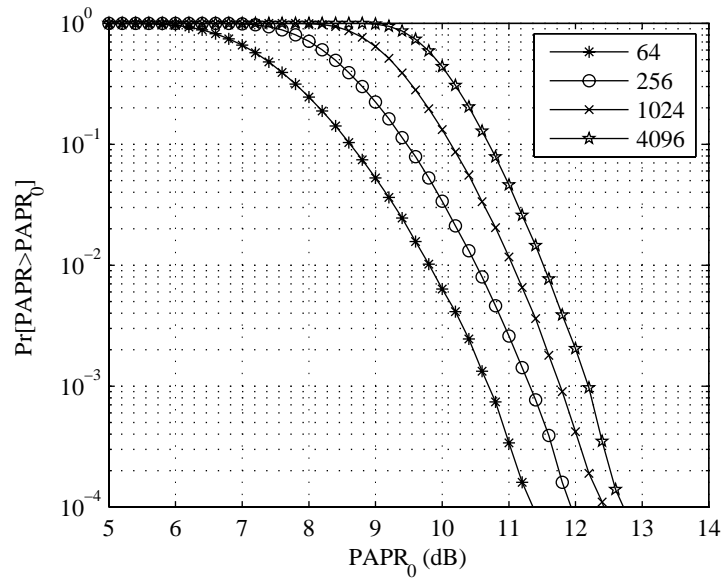
Figure 4.3. PAPR CCDF for a QPSK modulated OFDM system employing N subcarriers.
