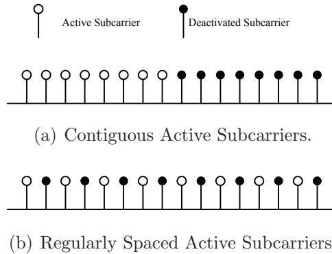
Figure 5.27. Subcarrier Distribution.
