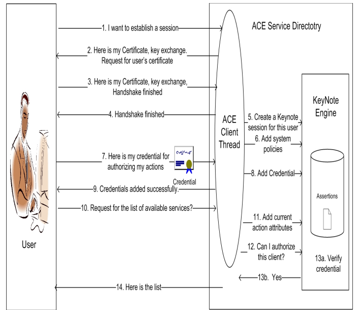
Fig. 3. Access Protocol showing the sequence of actions when an ACE Client contacts the Service Directory
