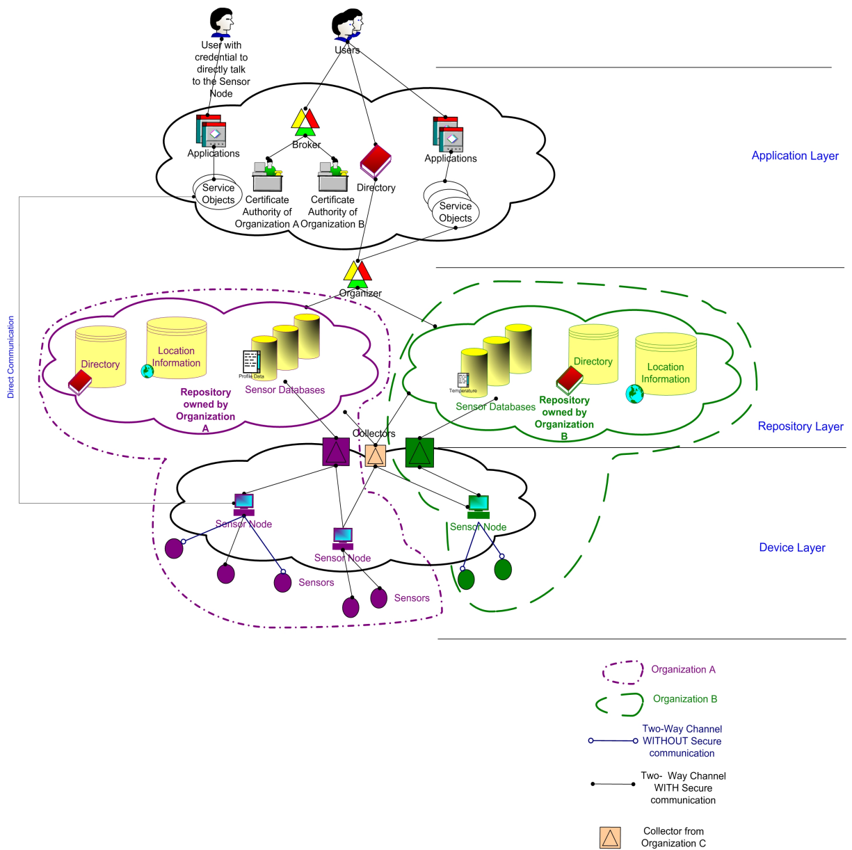
Fig. 1. Proposed Unified Multi-Ownership Sensor Network Architecture
