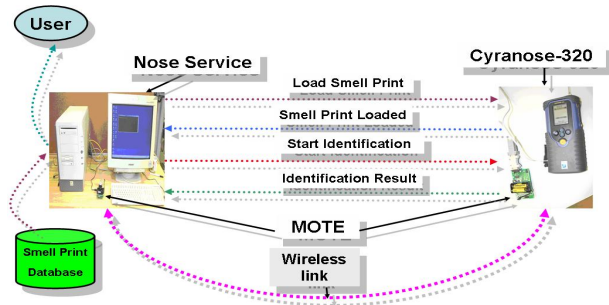
Fig. 5. Sequence of Message Exchange between Nose Server and Nose
